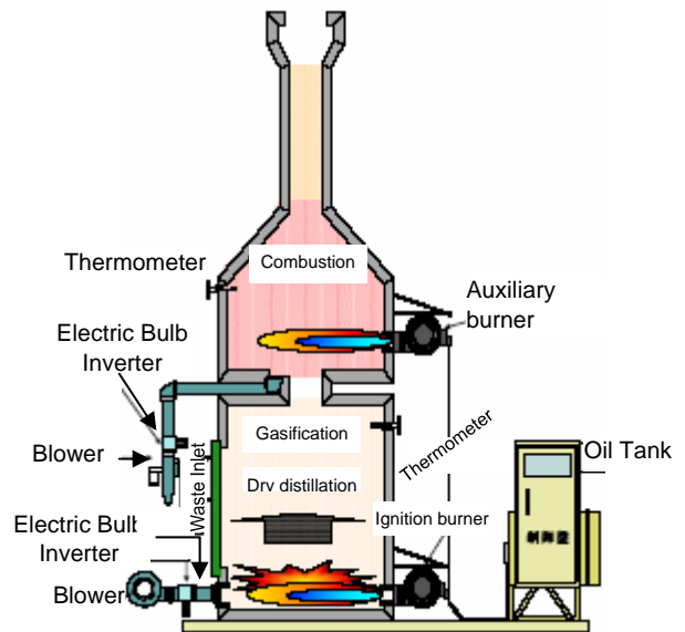
<Gasification/batch system>
